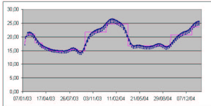
Figure 1: Gas Forward Curve
