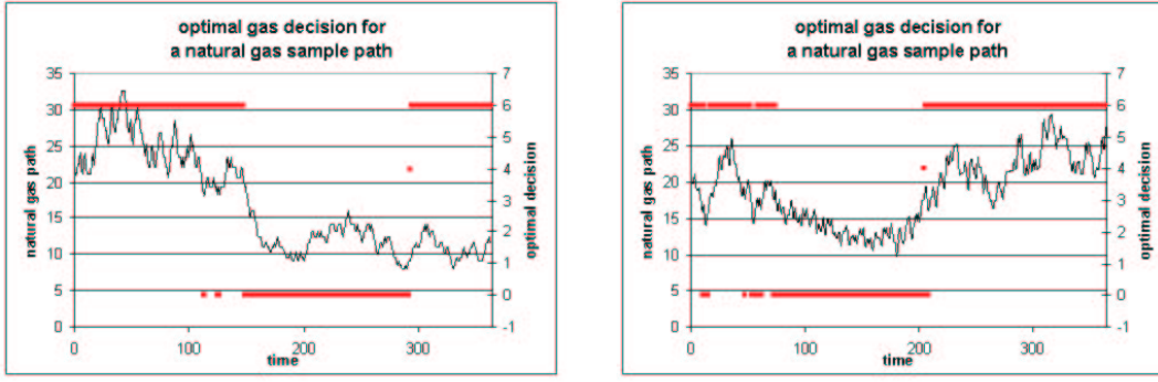
Figure 5: Swing contract. Optimal gas decision for a natural gas sample path. On the left, with a flat forward curve. On the right, with the real forward curve of Figure 1.
