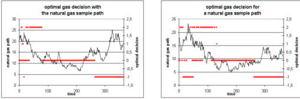
Figure 6: Storage contract. Optimal gas decision for a natural gas sample path. On the left, with a flat forward curve. On the right, with the real forward curve of Figure 1.
