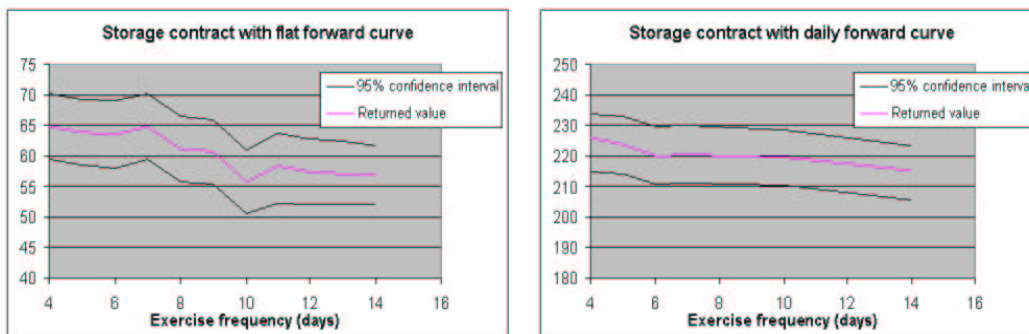
Figure 7: Flat forward curve on the left. Real forward curve on the right.
