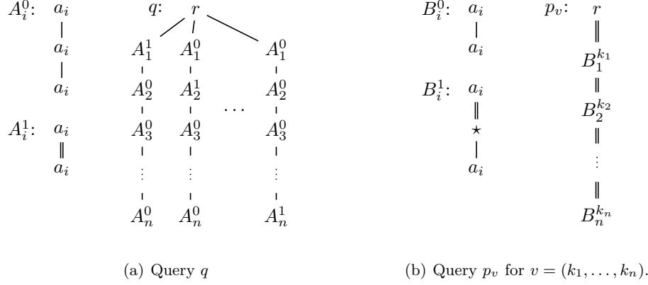
■ Figure 2 Twig query q requiring exponentially many examples w.r.t. p_v .
