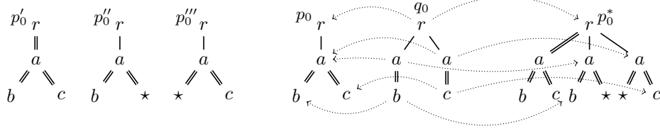
■ Figure 11 Immediate anchored generalizations versus an embedding with overlap p_0 \preceq q_0 .
