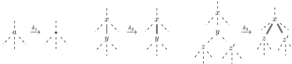
■ Figure 5 One-step generalization operations ( \rightarrow ).
