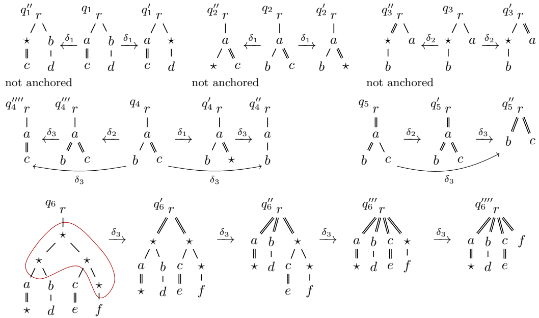
■ Figure 7 Applying generalization operations to anchored twig queries.
