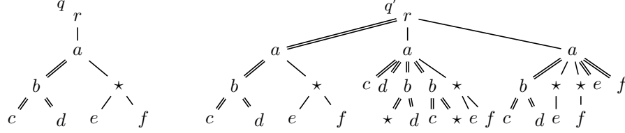
■ Figure 12 Constructing the minimal generalization q' of a query q ( q \triangleleft q' ).
