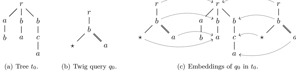
■ Figure 1 Tree, twig query, and embeddings.
