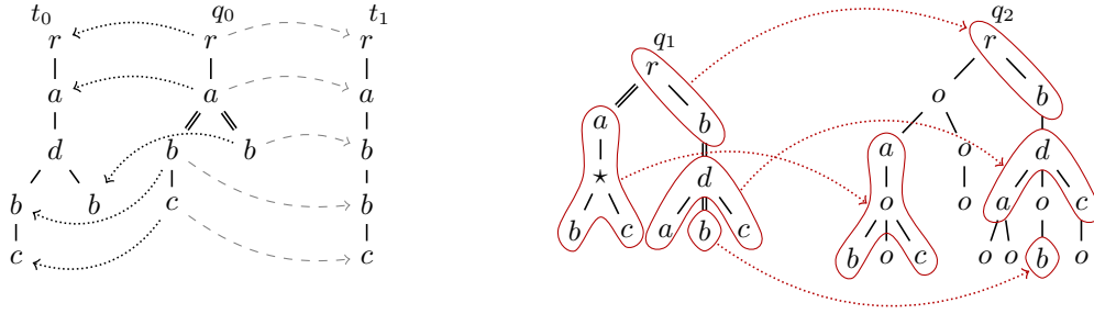
■ Figure 6 Injective embeddings t_0 \preceq_\circ q_0 and q_2 \preceq_\circ q_1 .
